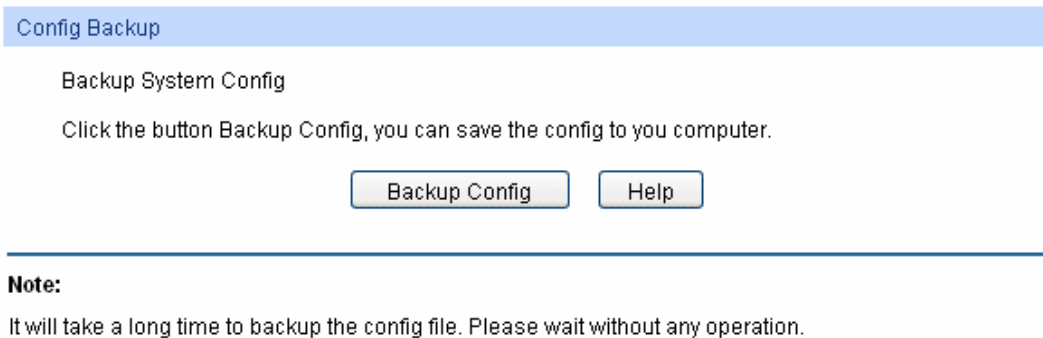
Figure 4-11 Config Backup
